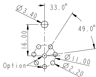
Recommended PCB Layout Tolerance \pm 0.05 ANGLES \pm 1^\circ
