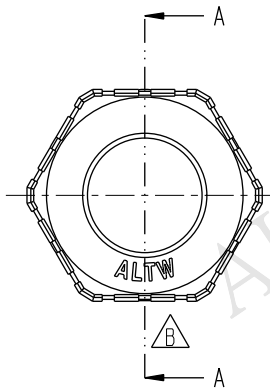
2 Clamping Nut
