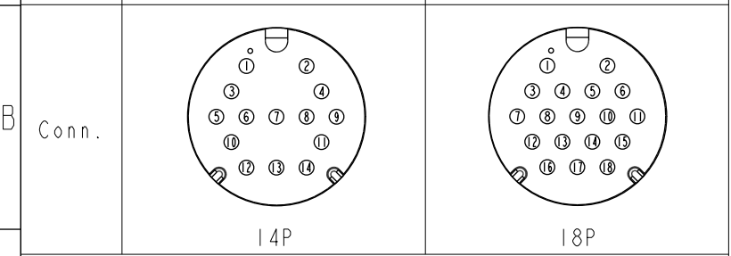
△B Pin Assignments Front View
