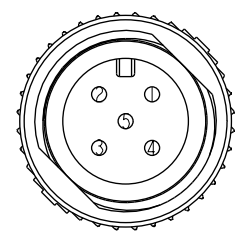
Conn.4 Pin Assignments Front View
