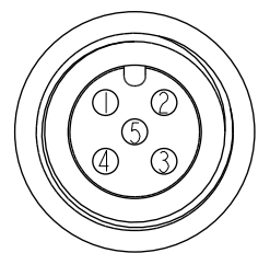
Conn.1&2&3 Pin Assignments Front View
