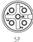
Pin Assignment Front View
