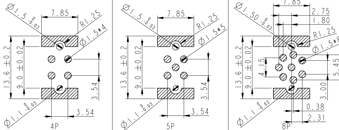
PCB Layout
